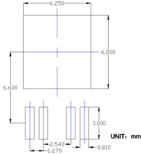
SUGGESTED SOLDER PAD LAYOUT
