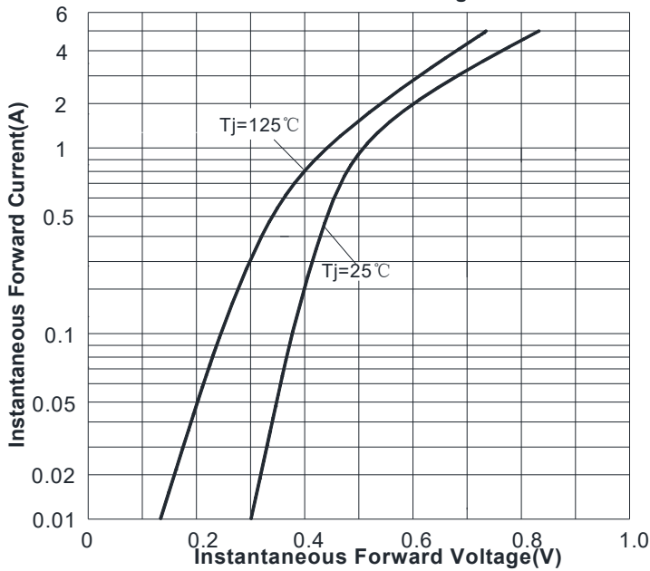
FIG3: Forward Voltage
